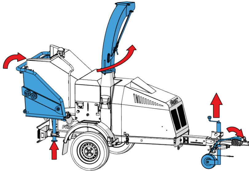
Figure 24 - Position de remorquage
